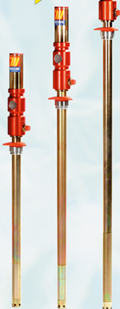
Pompe à huile R = 3:1 - 30 l/min • Long. 740mm Art. 020-1190-000 • Long. 940mm Art. 020-1195-000 • Long. 1250mm Art. 020-1196-000
